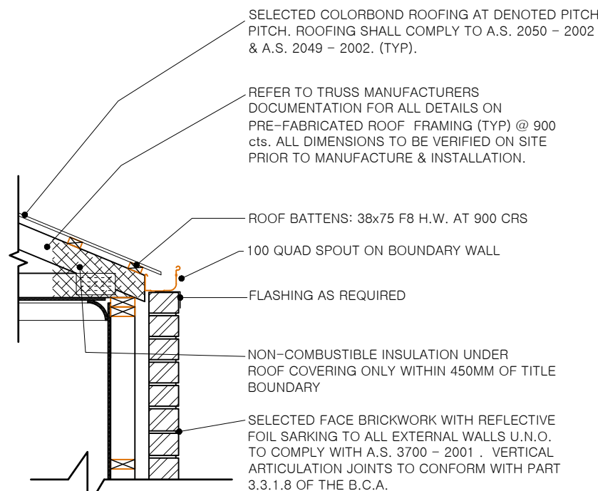
GUTTER ON BRICKWORK DETAIL SCALE 1:20
