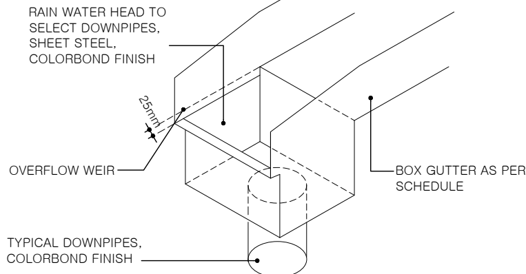
RAIN WATER HEAD DETAIL SCALE 1:10
