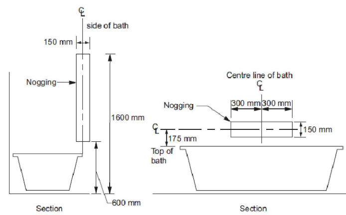
Figure 6.2b: Location of sheeting for walls surrounding a bath
