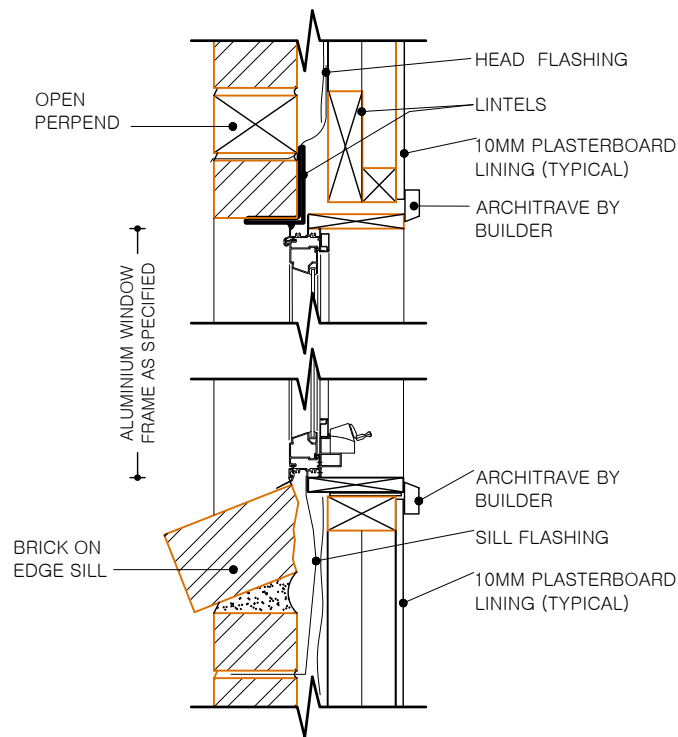
WINDOW DETAIL SCALE 1:20
