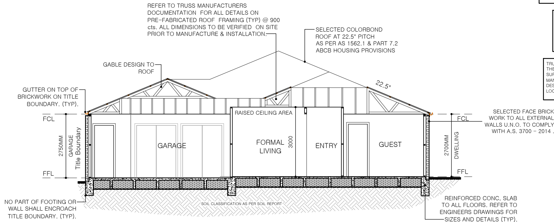
SECTION A SCALE 1:100
