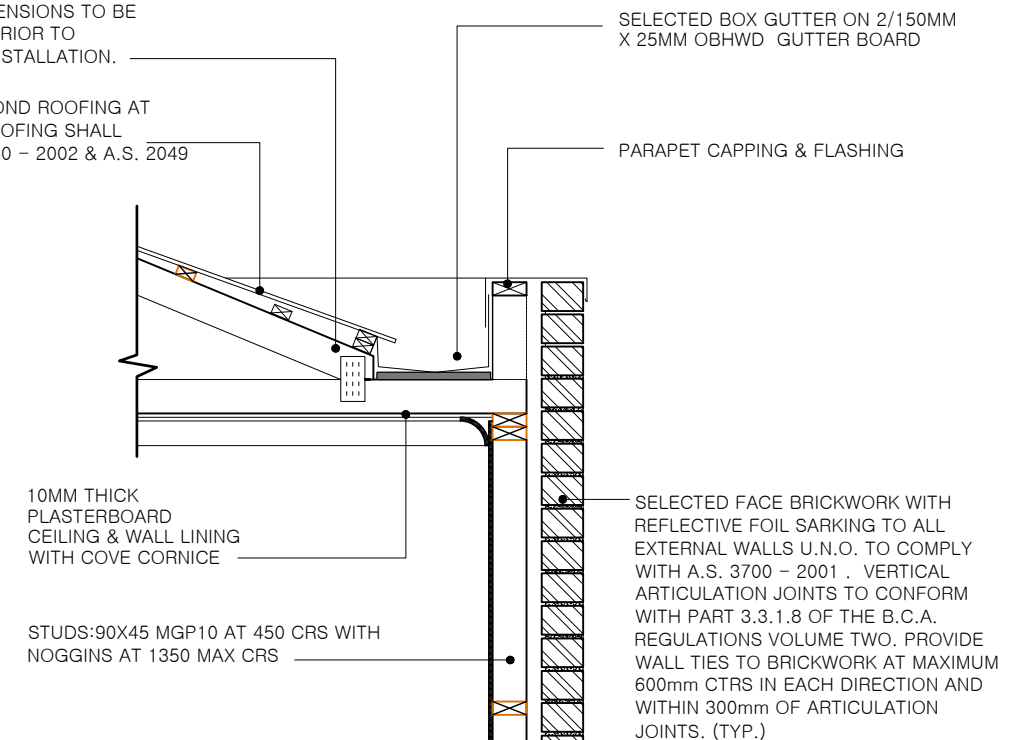
BOX GUTTER DETAIL-BRICK SCALE 1:20
