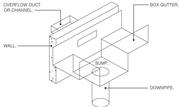
SUMP DETAIL NOT TO SCALE
