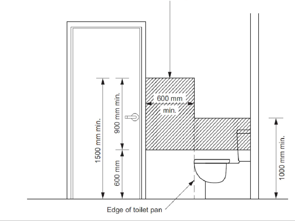
Figure 6.2e: Minimum extent of sheeting for wall adjacent to a toilet pan Minimum extent of structural sheeting clear of any door frame, window frame or wall opening
