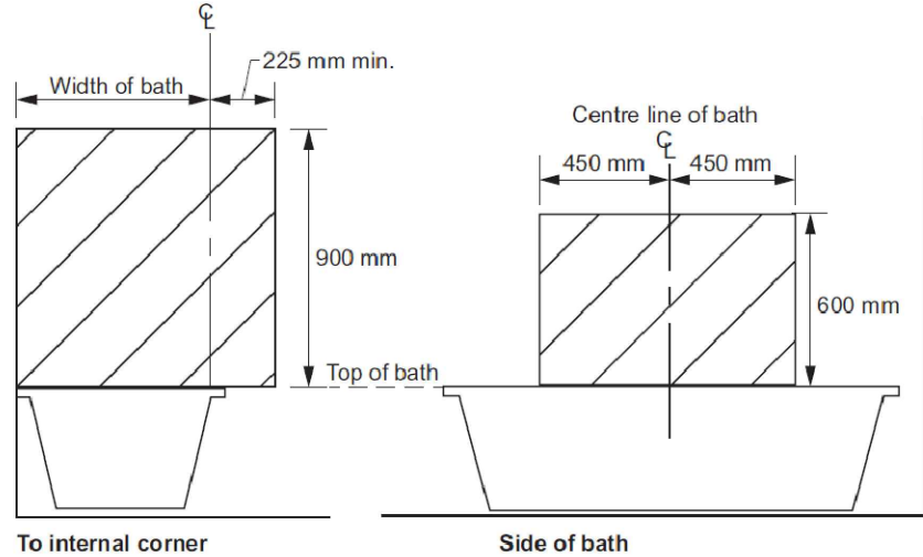
Figure 6.2c: Location of noggings for shower walls
